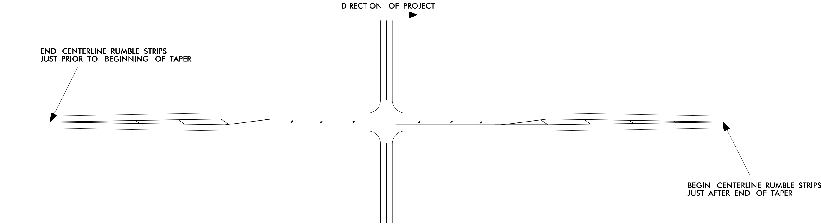
LEFT TURN LANE RUMBLE STRIP DETAIL USE DETAIL FOR ALL LEFT TURN LANE TAPERS
